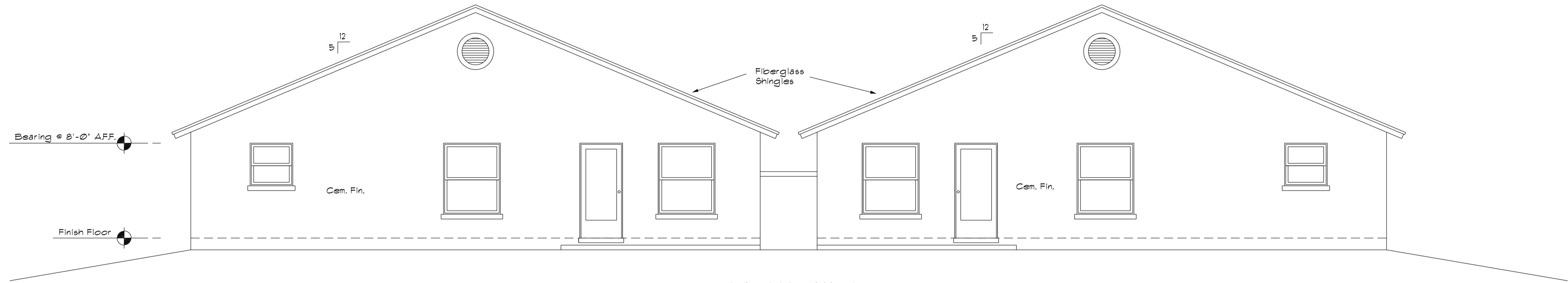
REAR ELEVATION
